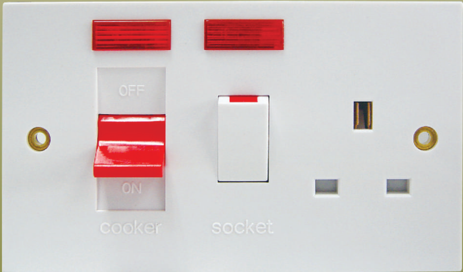
B2148L 45A Cooker Control Unit + 13A Switched Socket with neon
